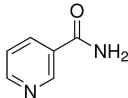
NIACIN AMIDE
